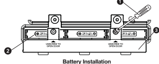
Battery Installation
