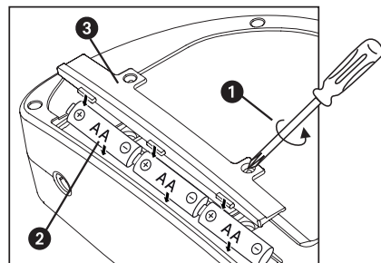
Battery Installation
